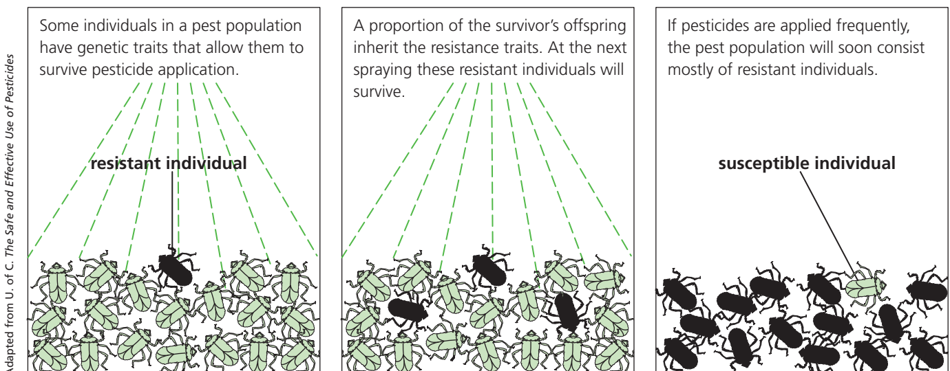
Figure 1.4 Pesticide resistance
